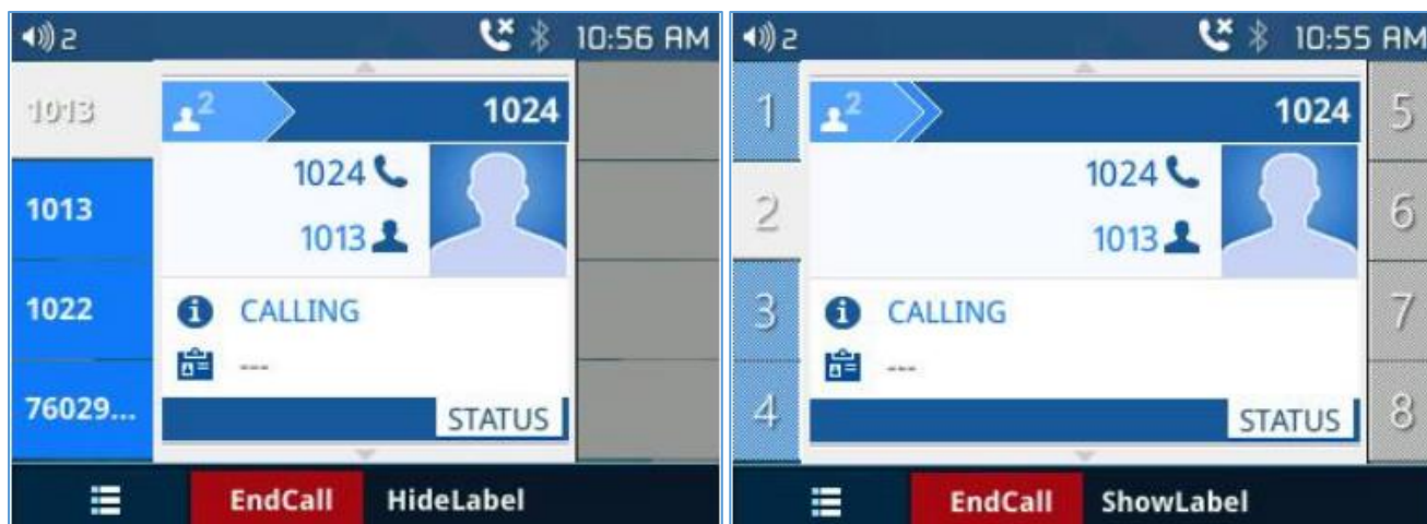
Figure 35: Show/Hidden Labels
