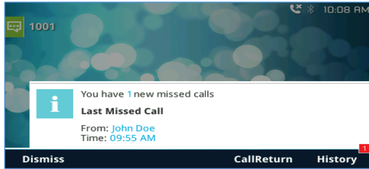
Figure 70: Missed Calls
